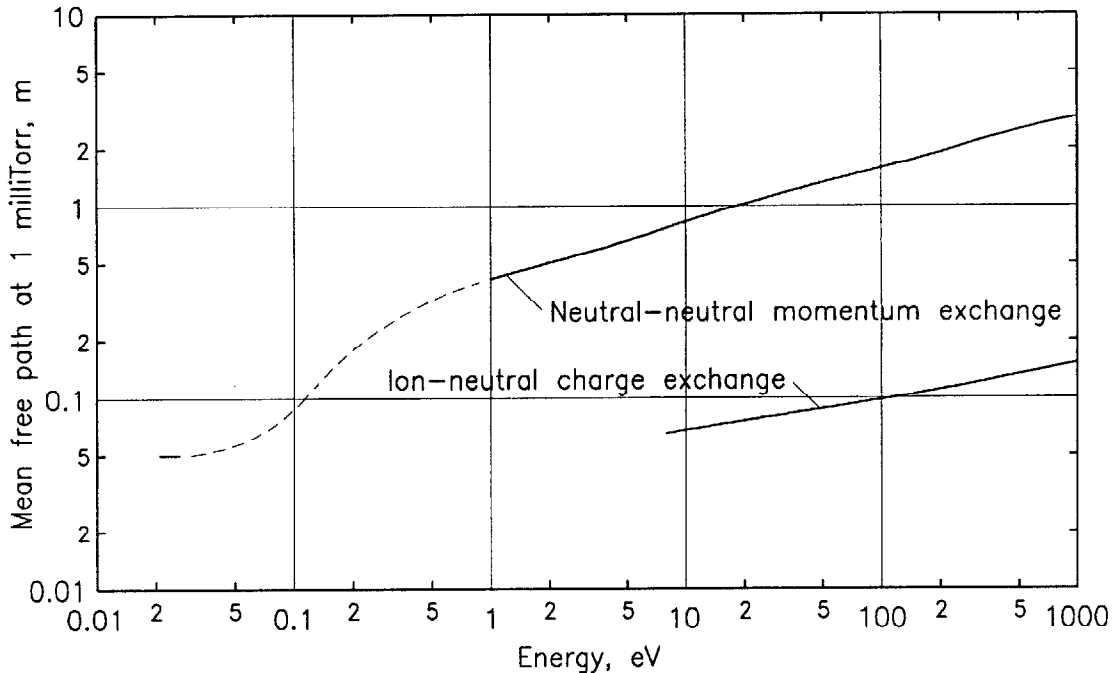
Fig. 1. Charge-exchange and momentum-exchange path lengths for argon.
